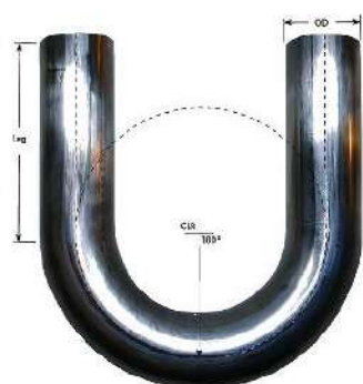
U bend tube, Heat Exchanger U Bend Tube
